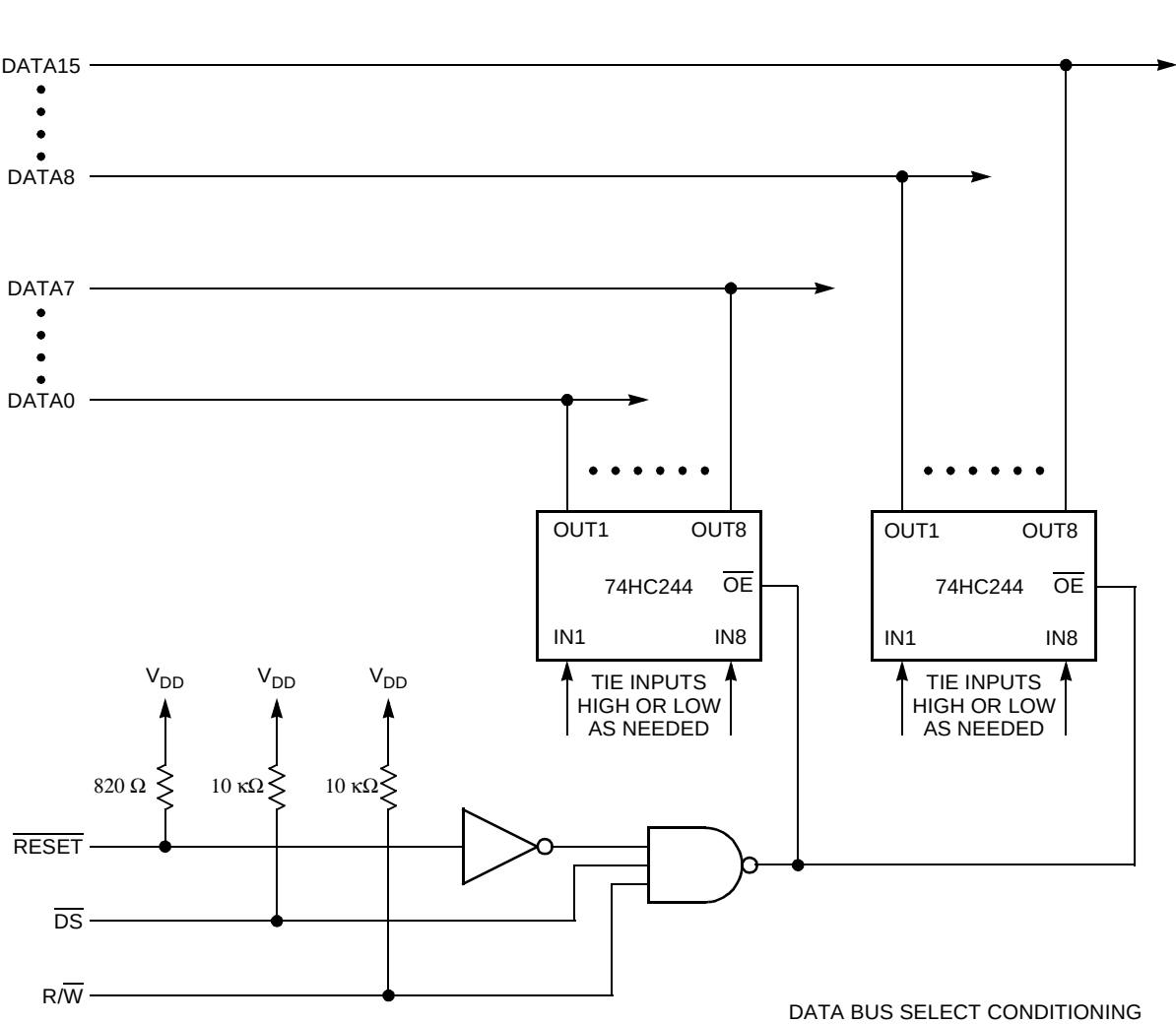
Figure 4-19 Preferred Circuit for Data Bus Mode Select Conditioning
