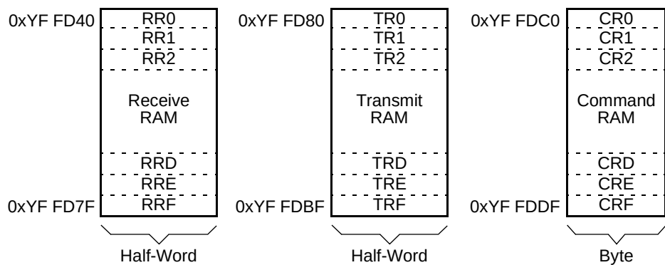
Figure 6-3 QSPI RAM
