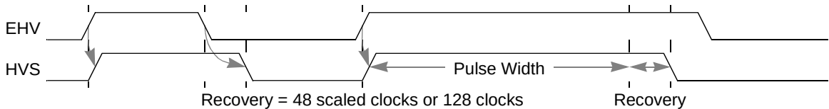
Figure 10-4 Pulse Status Timing
