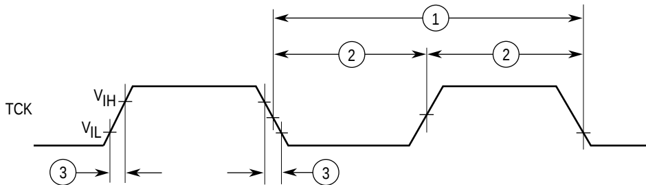
Figure 11-19. Test Clock Input Timing Diagram
