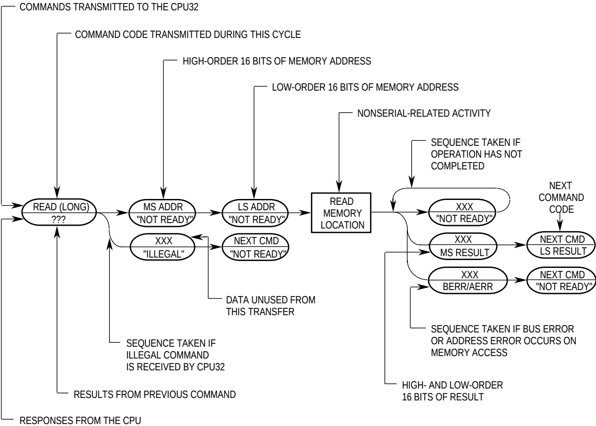
Figure 5-27. Command-Sequence Diagram
