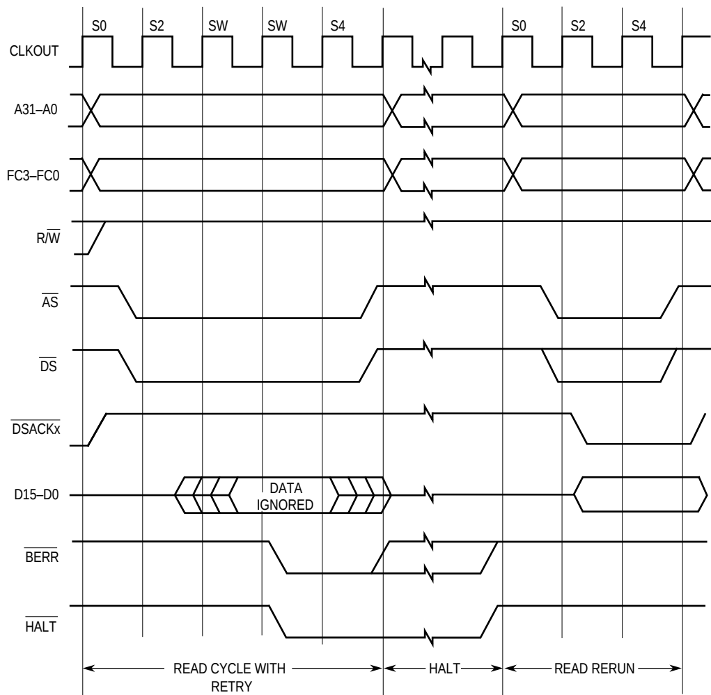
Figure 3-19. Retry Sequence
