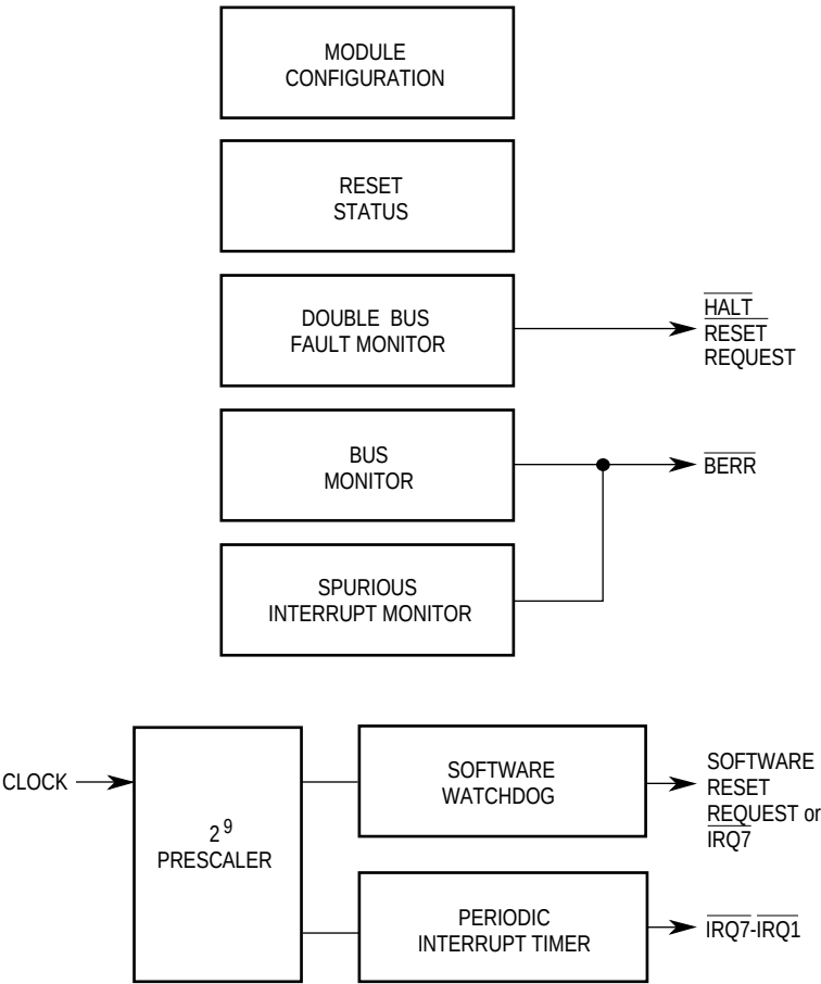
Figure 4-2. System Configuration and Protection Function
