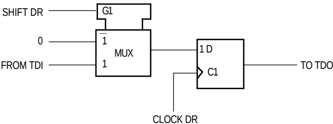
Figure 9-9. Bypass Register
