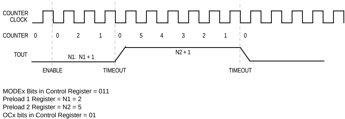
Figure 8-7. Variable-Width Single-Shot Pulse Generator Mode
