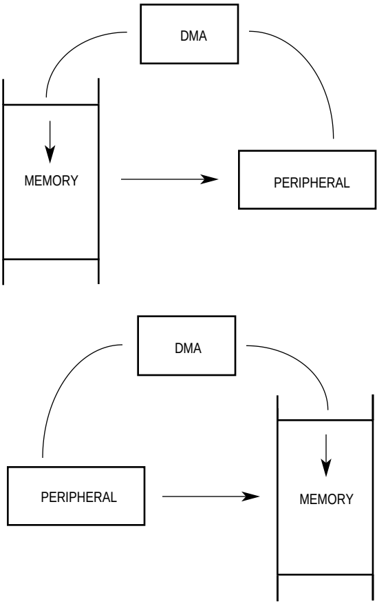
Figure 6-2. Single-Address Transfers
