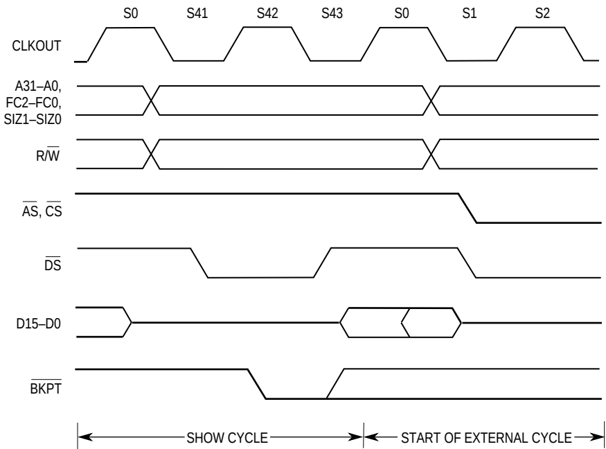
Figure 3-26. Show Cycle Timing Diagram
