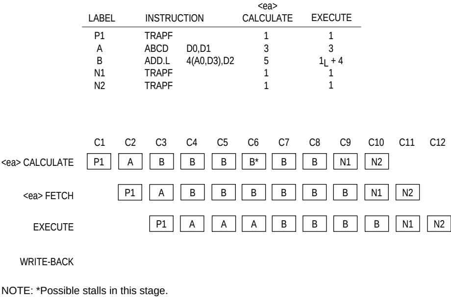
Figure 10-3. Interlocked Stages
