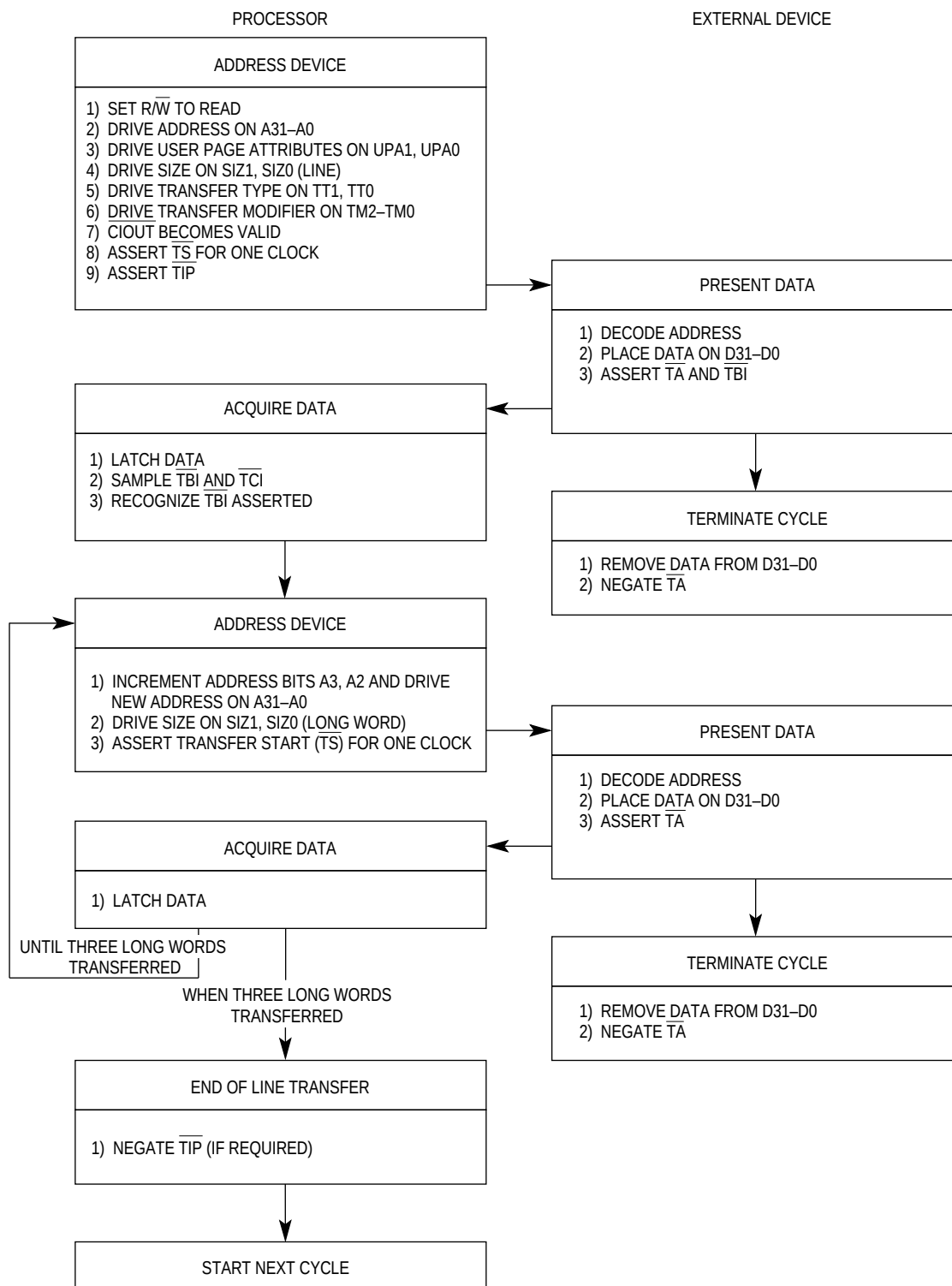
Figure 7-12. Burst-Inhibited Line Read Transfer Flowchart
