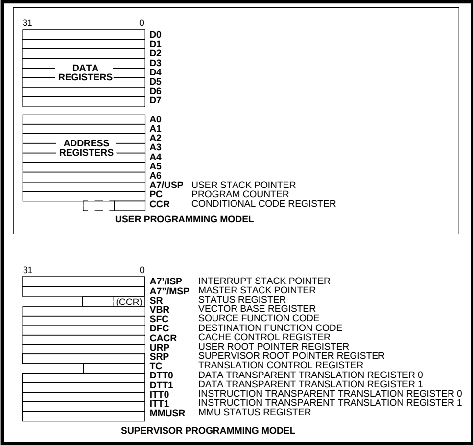
Figure A-2. MC68LC040 Programming Model
