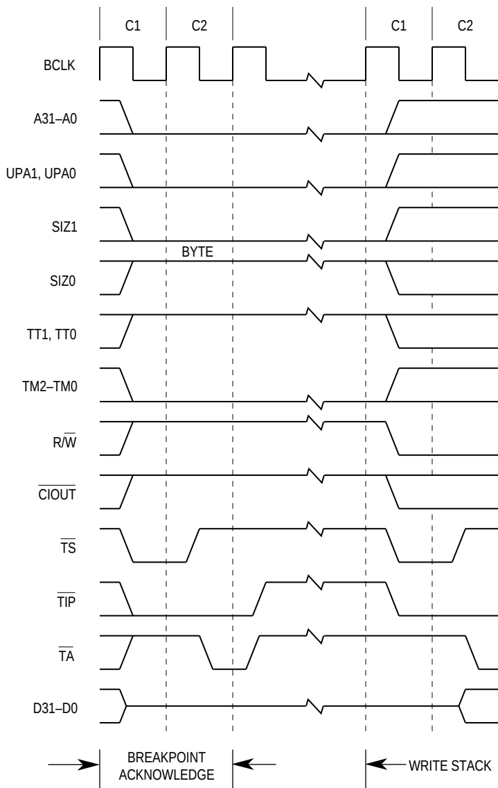
Figure 7-25. Breakpoint Interrupt Acknowledge Bus Cycle Timing
