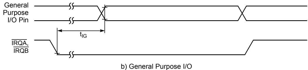
Figure 10-7 External Level-Sensitive Interrupt Timing
