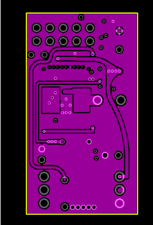
Figure 35. PCB Layer 2
