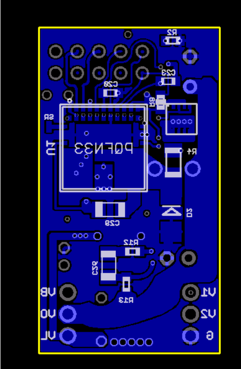
Figure 37. PCB Layer 4
