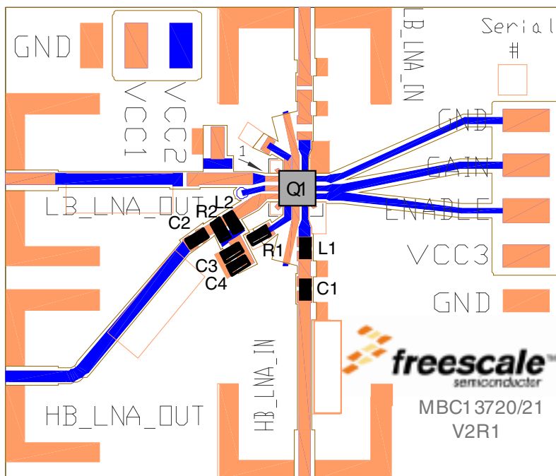
Figure 13. Front Side
