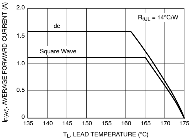
Figure 5. Current Derating
