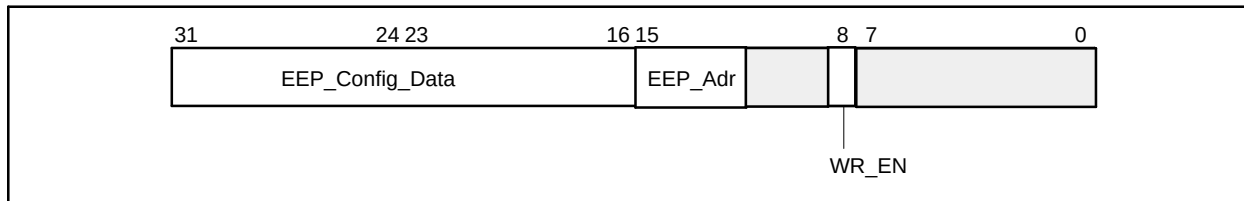
Fig. 7.4.1 EEPROM configuration Register
