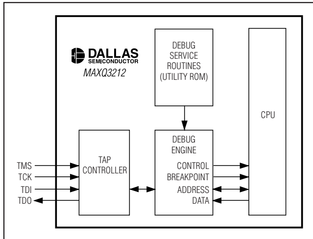
Figure 5. In-Circuit Debugger
