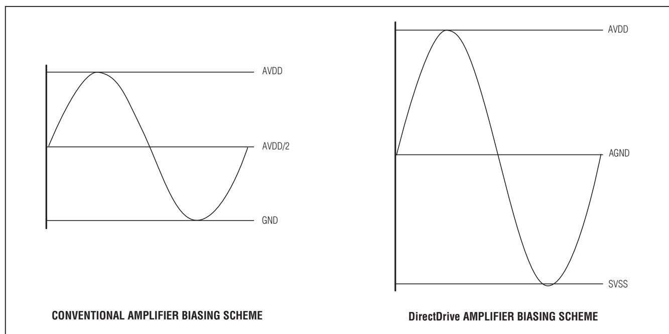
Figure 4. Traditional Amplifier Output vs. MAX9856 DirectDrive Output
