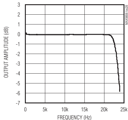
ADC DIGITAL FILTER FREQUENCY RESPONSE
