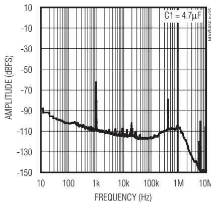
WIDEBAND FFT, DAC TO HP AMP, 48kHz SYNCHRONOUS MASTER MODE, -60dBFS
