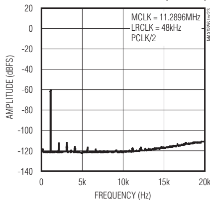
FFT, LINE IN TO ADC (48kHz) ASYNCHRONOUS SLAVE MODE (-60dBFS)
