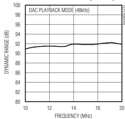
DYNAMIC RANGE vs. MCLK FREQUENCY (-60dBFS)
