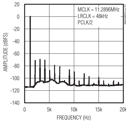
FFT, LINE IN TO ADC (48kHz) ASYNCHRONOUS SLAVE MODE (0dBFS)
