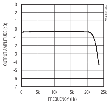
DAC DIGITAL FILTER FREQUENCY RESPONSE
