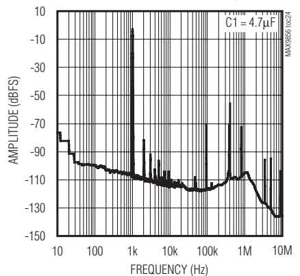
WIDEBAND FFT, DAC TO HP AMP, 48kHz SYNCHRONOUS MASTER MODE, 0dBFS
