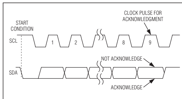
Figure 10. Acknowledge
