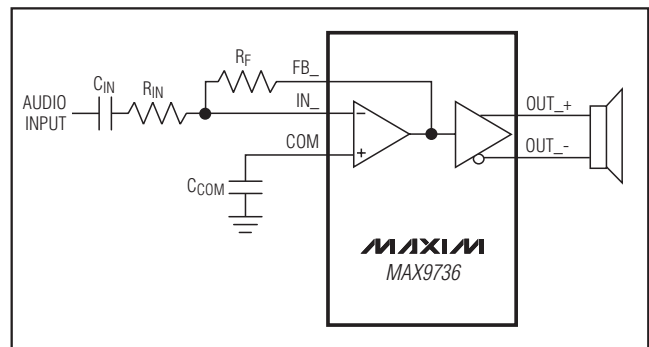
Figure 5. Setting Gain
