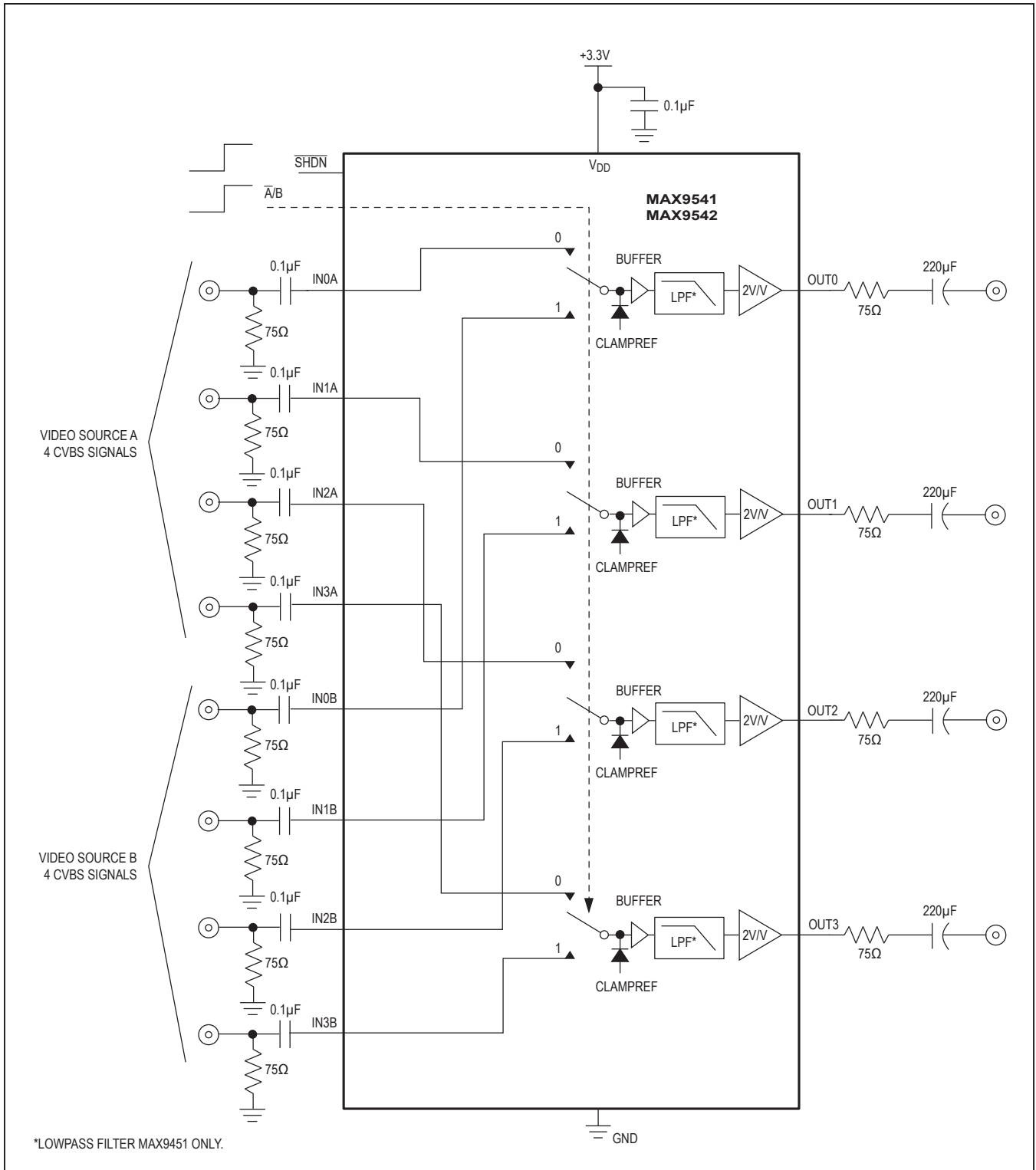
Figure 3. AC-Coupled Outputs
