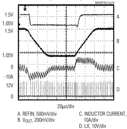
DYNAMIC OUTPUT-VOLTAGE TRANSITION (PWM MODE)
