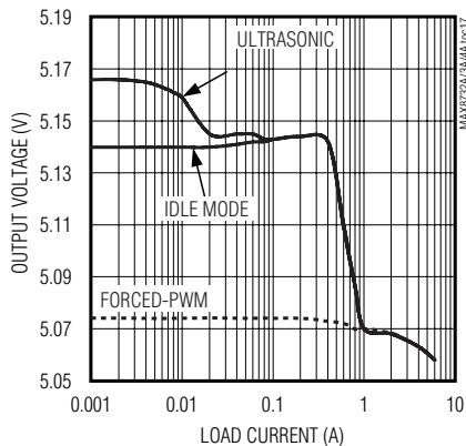
MAX8732A OUT5 VOLTAGE REGULATION vs. LOAD CURRENT
