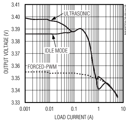
MAX8732A OUT3 VOLTAGE REGULATION vs. LOAD CURRENT
