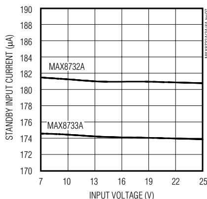
STANDBY INPUT CURRENT vs. INPUT VOLTAGE
