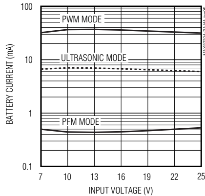
MAX8732A NO-LOAD BATTERY CURRENT vs. INPUT VOLTAGE
