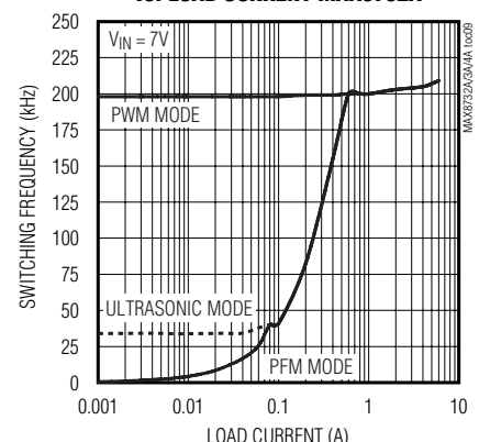
MAX8732A 5V OUTPUT SWITCHING FREQUENCY vs. LOAD CURRENT
