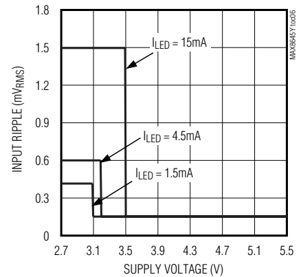
INPUT RIPPLE VOLTAGE vs. SUPPLY VOLTAGE WITH SIX MAIN LEDs
