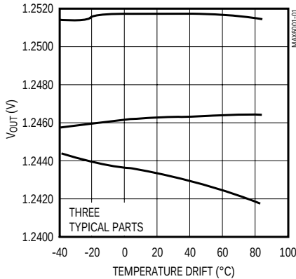
MAX6001 OUTPUT VOLTAGE TEMPERATURE DRIFT
