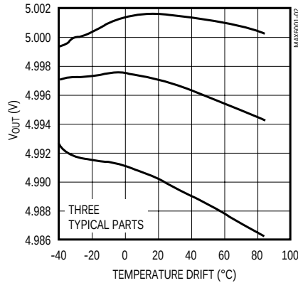
MAX6005 OUTPUT VOLTAGE TEMPERATURE DRIFT
