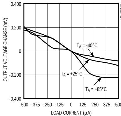
MAX6005 LOAD REGULATION
