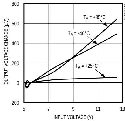
MAX6005 LINE REGULATION
