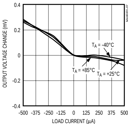
MAX6001 LOAD REGULATION
