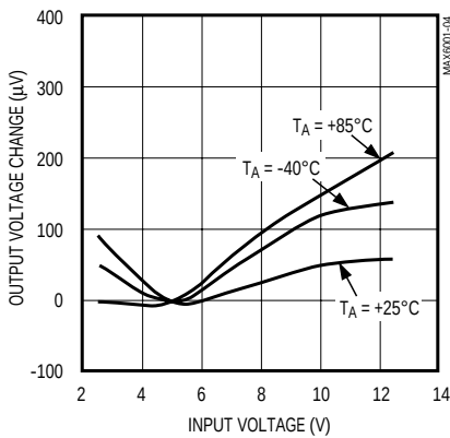
MAX6001 LINE REGULATION
