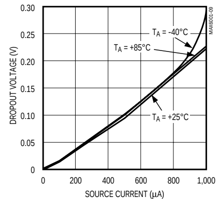
MAX6004/MAX6005 DROPOUT VOLTAGE vs. SOURCE CURRENT
