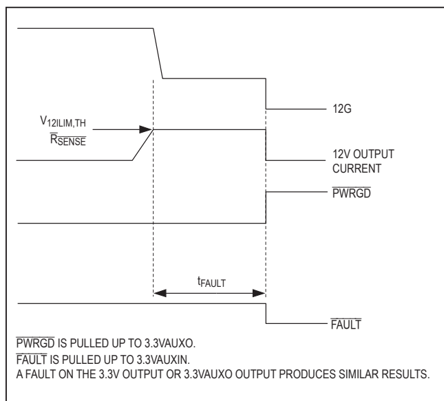
Figure 4. 12V Output Overcurrent/Short Circuit During Normal Operation
