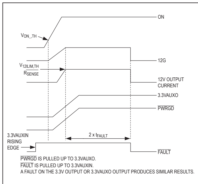
Figure 3. 12V Power-Up Timing (Turn-On into Output Overcurrent/Short Circuit)
