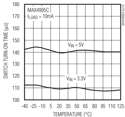
SWITCH TURN-ON TIME vs. TEMPERATURE
