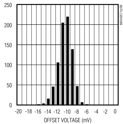
OFFSET VOLTAGE HISTOGRAM
