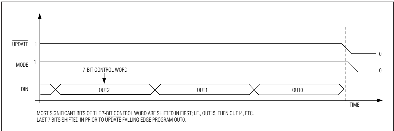
Figure 5. Mode 1: Complete Matrix Mode Programming
