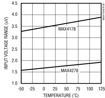
INPUT VOLTAGE RANGE vs. TEMPERATURE
