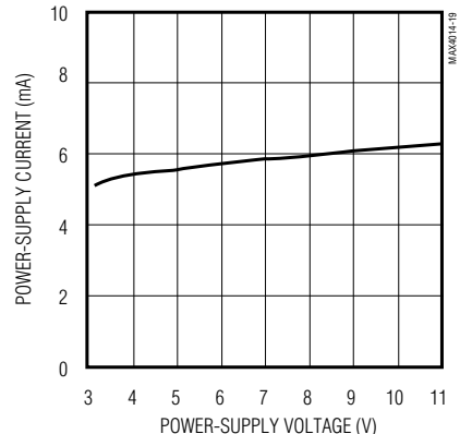
POWER-SUPPLY CURRENT (PER AMPLIFIER) vs. POWER-SUPPLY VOLTAGE
