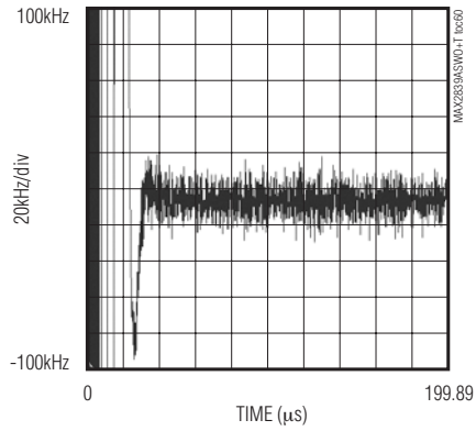
Rx-TO-Tx TURNAROUND FREQUENCY GLITCHING SETTling
