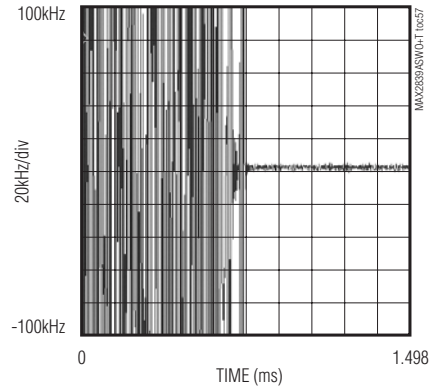
CHANNEL-SWITCHING FREQUENCY SETTLING (2.7GHz TO 2.3GHz, MANUAL VCO SUB-BAND SELECTION)
