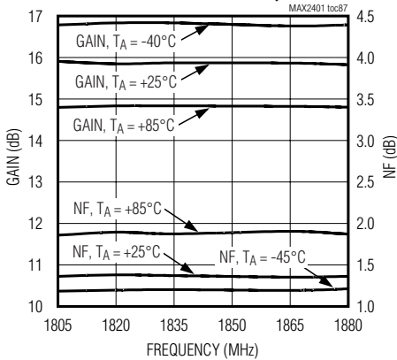
LNA GAIN AND NF vs. FREQUENCY
