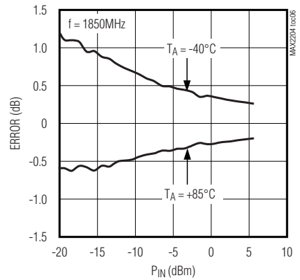
DETECTOR ERROR FROM T_A = +25^\circ C AT 1850MHz
