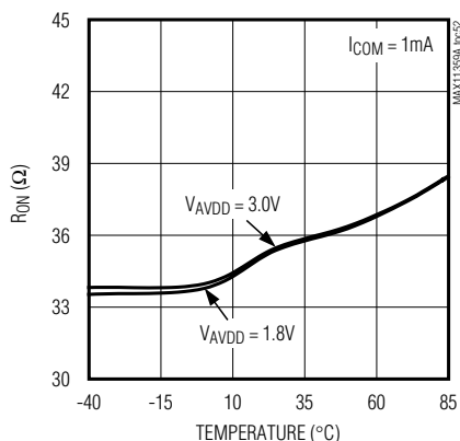
SPDT ON-RESISTANCE vs. TEMPERATURE
