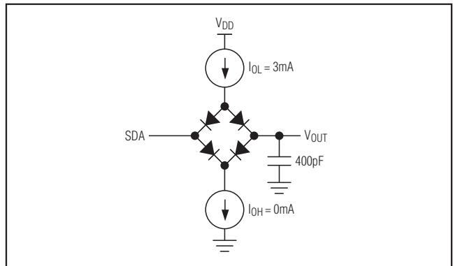
Figure 2. Load Circuit
