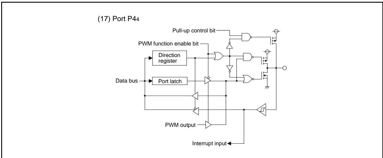
Fig 12. Port block diagram (3)
