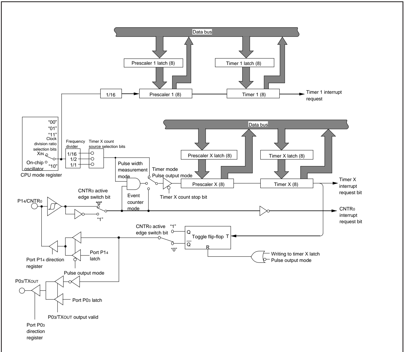
Fig. 24 Block diagram of timer 1 and timer X
