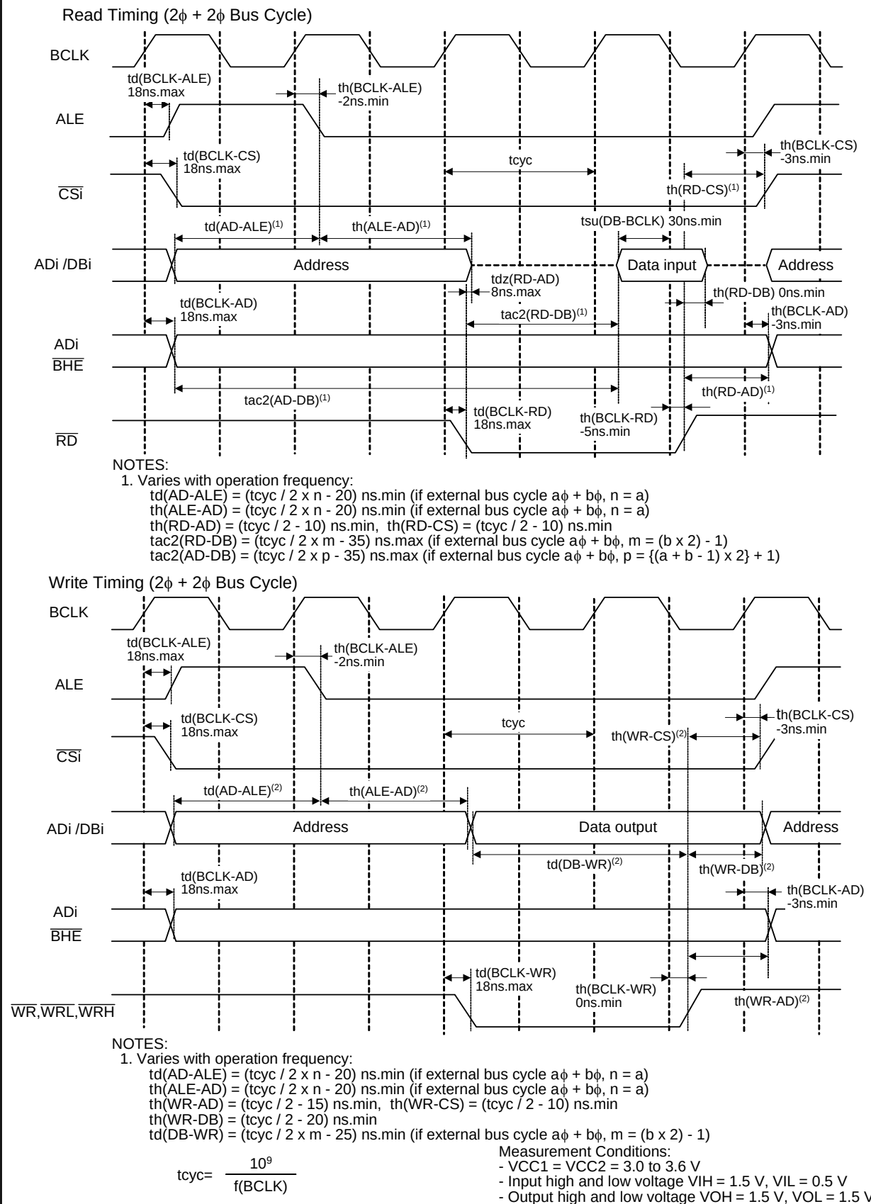
Figure 5.10 VCC1 = VCC2 = 3.3 V Timing Diagram (4/4)
