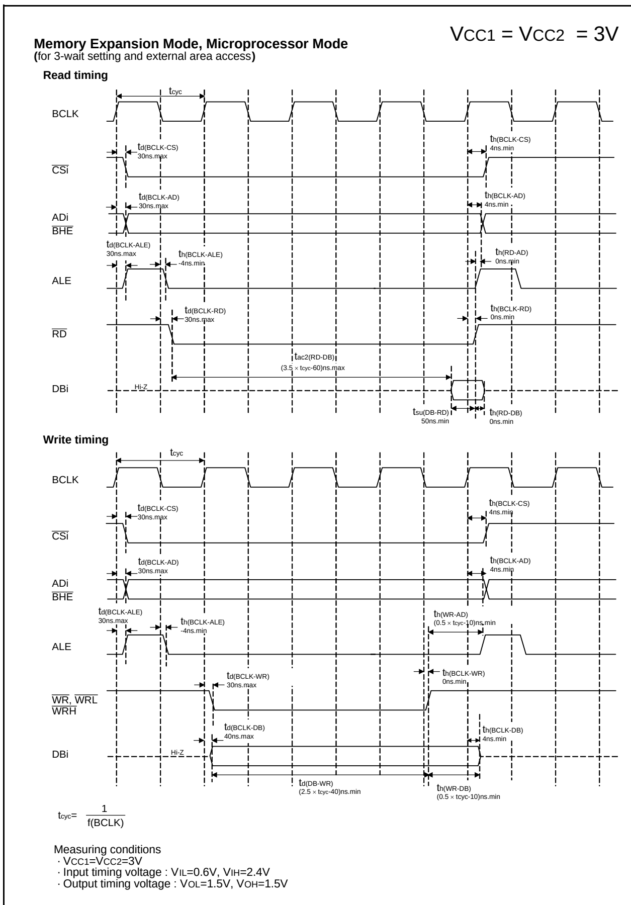
Figure 5.19 Timing Diagram (7)
