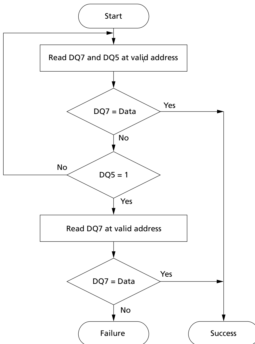
Figure 6: Data Polling Flowchart
