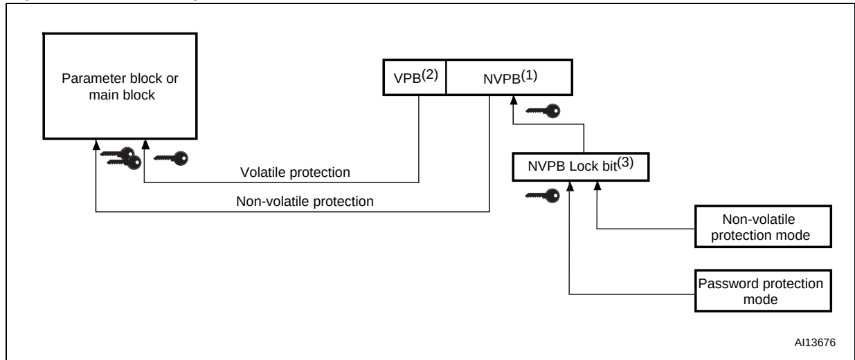
Figure 6. Software protection scheme
