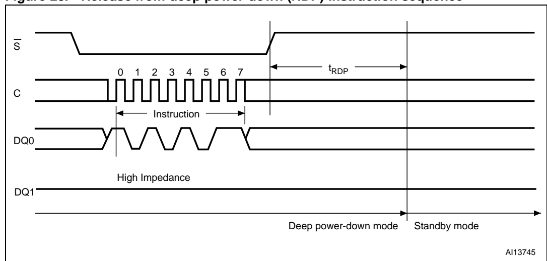
Figure 28. Release from deep power-down (RDP) instruction sequence
