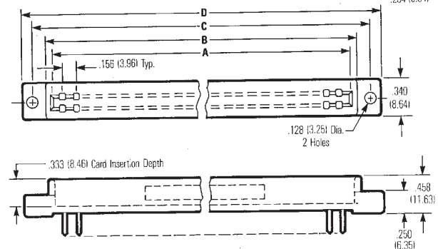
With Plain Mounting Holes
