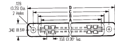
With Plain Mounting Holes
