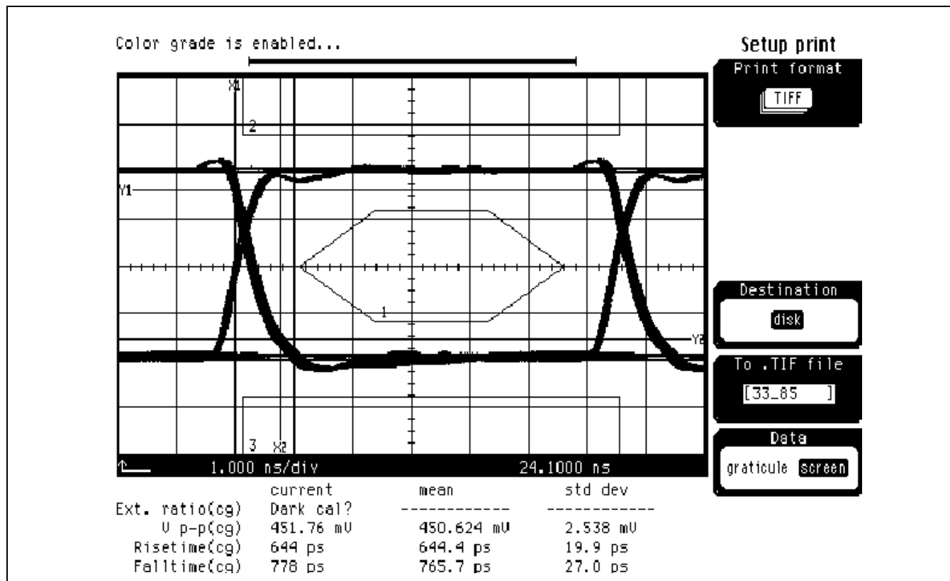
Figure 3-3. Eye Diagram
