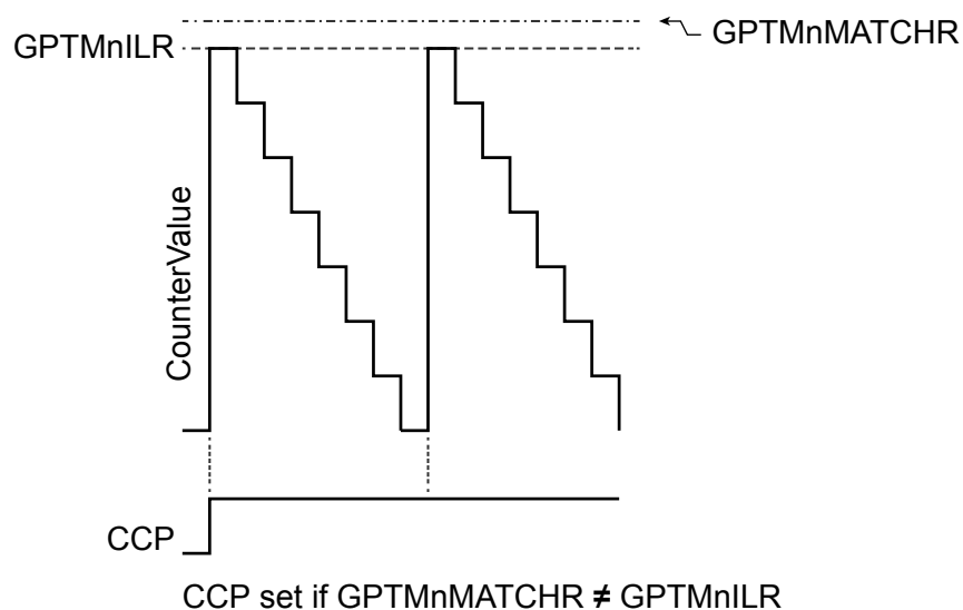
Figure 10-6. CCP Output, GPTMTnMATCHHR > GPTMTnILR
