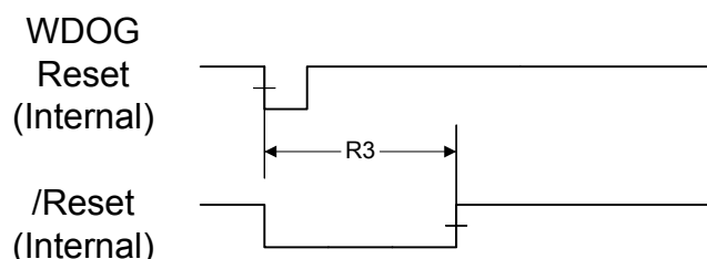
Figure 24-10. Watchdog Reset Timing
