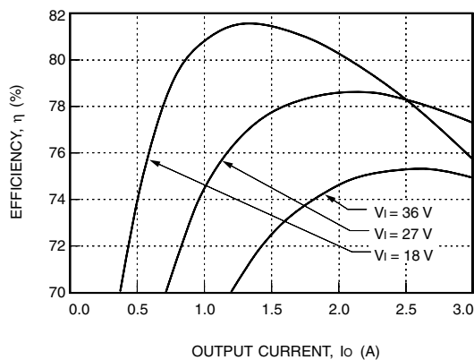
Figure 18. LC015F Typical Efficiency vs. Output Current at T_c = 25 °C
