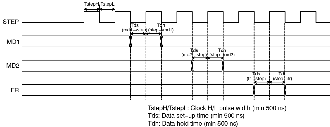
Figure 6. Input Timing
