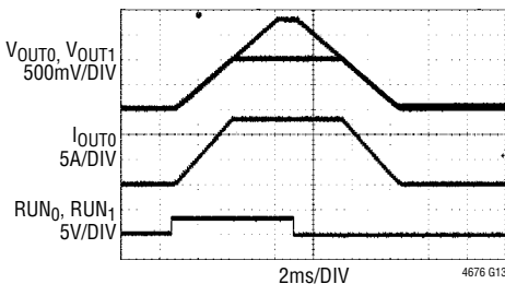
FIGURE 44 CIRCUIT AT 12\text{V}_{\text{IN}} , 77mΩ LOAD ON \text{V}_{\text{OUT}0} , NO LOAD ON \text{V}_{\text{OUT}1} . \text{TON\_RISE}_0 = 3\text{ms} , \text{TON\_RISE}_1 = 5.297\text{ms} , \text{TOFF\_DELAY}_1 = 0\text{ms} , \text{TOFF\_DELAY}_0 = 2.43\text{ms} , \text{TOFF\_FALL}_1 = 5.328\text{ms} , \text{TOFF\_FALL}_0 = 3\text{ms} , \text{ON\_OFF\_CONFIG}_n = 0x1E
