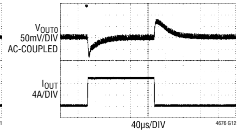
FIGURE 44 CIRCUIT AT 24\text{V}_{\text{IN}} , \text{C}_{\text{OUT}0} = 5 \times 100\mu\text{F} AND \text{V}_{\text{OUT}0} COMMANDED TO 3.300V. 0A TO 10A LOAD STEP AT 10A/µs
