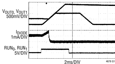
FIGURE 44 CIRCUIT AT 12\text{V}_{\text{IN}} , 77mΩ LOAD ON \text{V}_{\text{OUT}0} , 500Ω ON \text{V}_{\text{OUT}1} . \text{V}_{\text{OUT}1} PRE-BIASED THROUGH A DIODE. \text{TON\_RISE}_0 = 3\text{ms} , \text{TON\_RISE}_1 = 5.297\text{ms} , \text{TOFF\_DELAY}_1 = 0\text{ms} , \text{TOFF\_DELAY}_0 = 2.43\text{ms} , \text{TOFF\_FALL}_1 = 5.328\text{ms} , \text{TOFF\_FALL}_0 = 3\text{ms} , \text{ON\_OFF\_CONFIG}_1 = 0x1F , \text{ON\_OFF\_CONFIG}_0 = 0x1E
