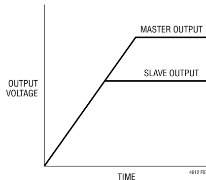
Figure 7. Coincident Output Tracking
