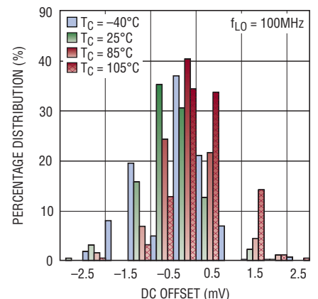
DC Offset Distribution, Q-Side
