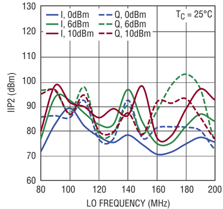
Uncalibrated IIP2 vs LO Power
