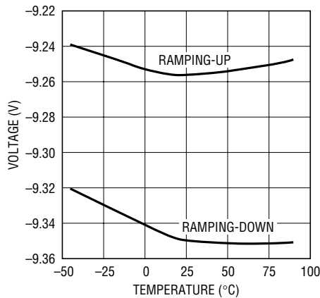
V EEIN Undervoltage Lockout vs Temperature
