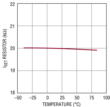
R IS ET vs Temperature
