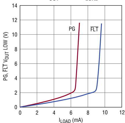
PG, FLT V_{OUT} Low vs I_{LOAD}
