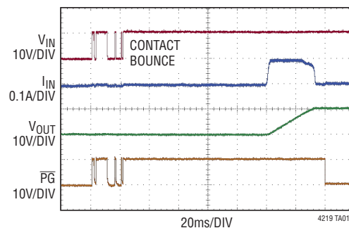
Power-Up Waveforms
