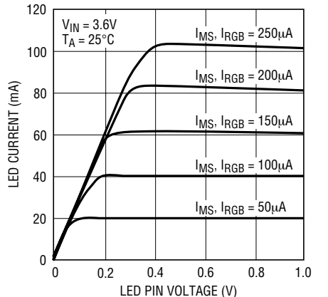
LED Pin Voltage for Higher LED Currents
