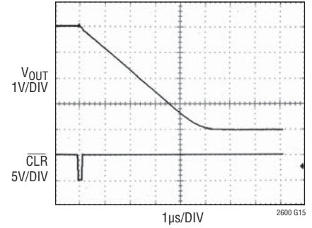
Hardware CLR
