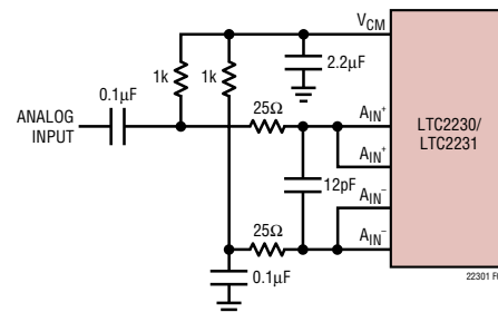
Figure 5. Single-Ended Drive
