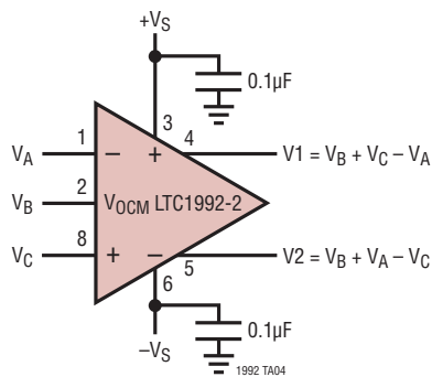
Zero Components, Single-Ended Adder/Subtractor
