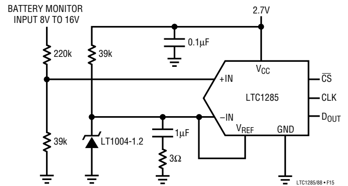
Figure 15. Micropower Battery Voltage Monitor
