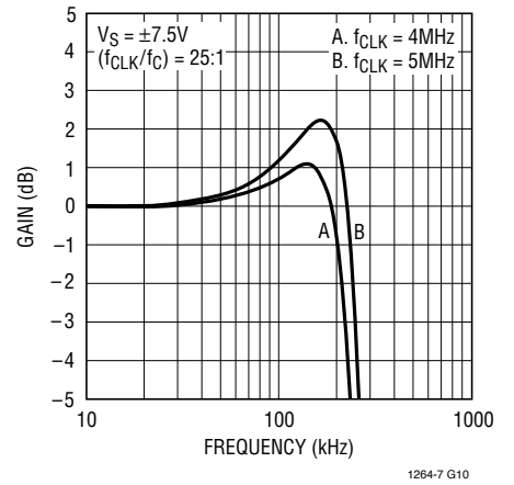
Passband Gain vs f_{CLK} at 85°C
